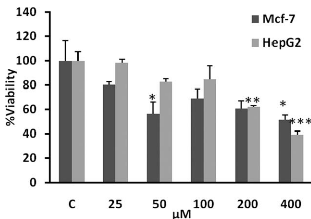
Figure 2. Dose-dependent growth inhibition of malignant cell lines by compounds 5b (25 to 400 μM) for 24 h. Viability was quantitated by MTT assay. The dose inducing 50% cell growth inhibition (IC 50 ) against Hep-G2 and MCF-7 was calculated 294.1 and 555.8 μM, respectively. Results are Mean ± SEM (n = 3). * P < 0.05, ** P < 0.01, and *** P < 0.001 compared with control (C).
